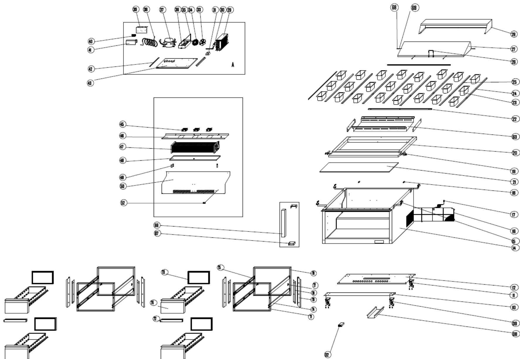
EXPLODE OF KCHMT60.24.4D
